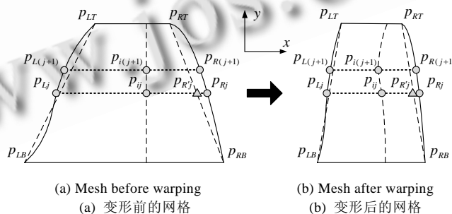
Fig.4 Horizontal warping of curve-edge trapezoid mesh
